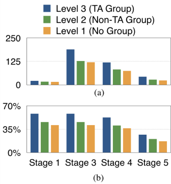
Figure 5: Code submissions from students receiving different levels of assistance. (a) Count of learning activities. (b) Average percentage of users achieved the learning stage.
